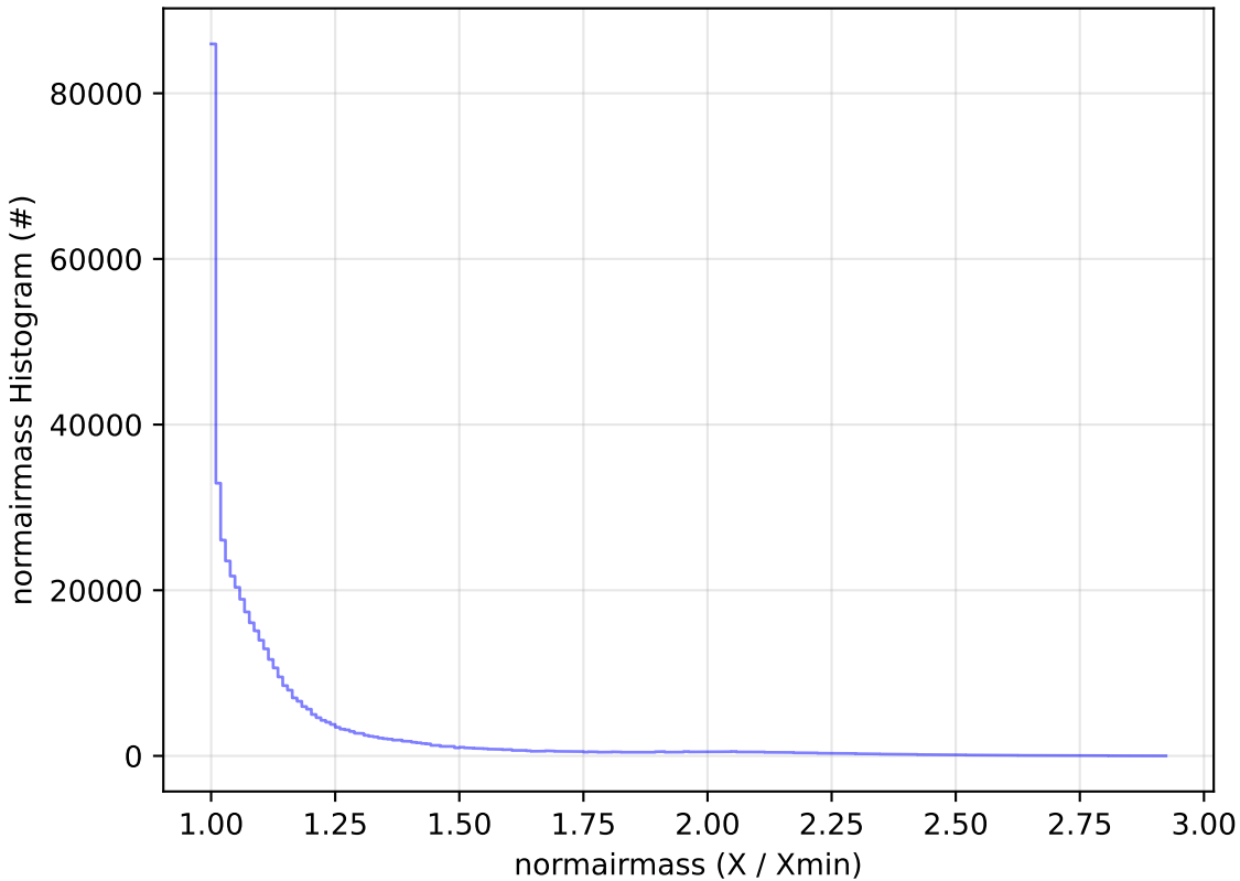
ddf_acor_sf10_lsf15_lsr10_v3.4_10yrs WFD i band: normairmass Histogram
