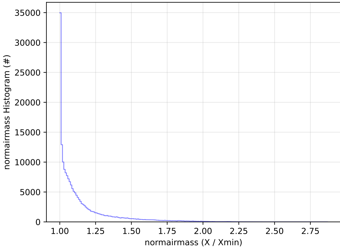
ddf_acor_sf10_lsf15_lsr10_v3.4_10yrs WFD g band: normairmass Histogram
