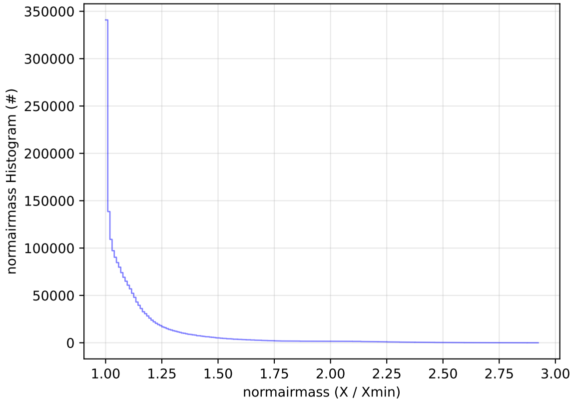
ddf_acor_sf10_lsf15_lsr10_v3.4_10yrs WFD all bands: normairmass Histogram
