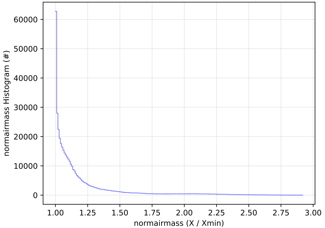
ddf_acor_sf10_lsf15_lsr10_v3.4_10yrs All sky z band: normairmass Histogram
