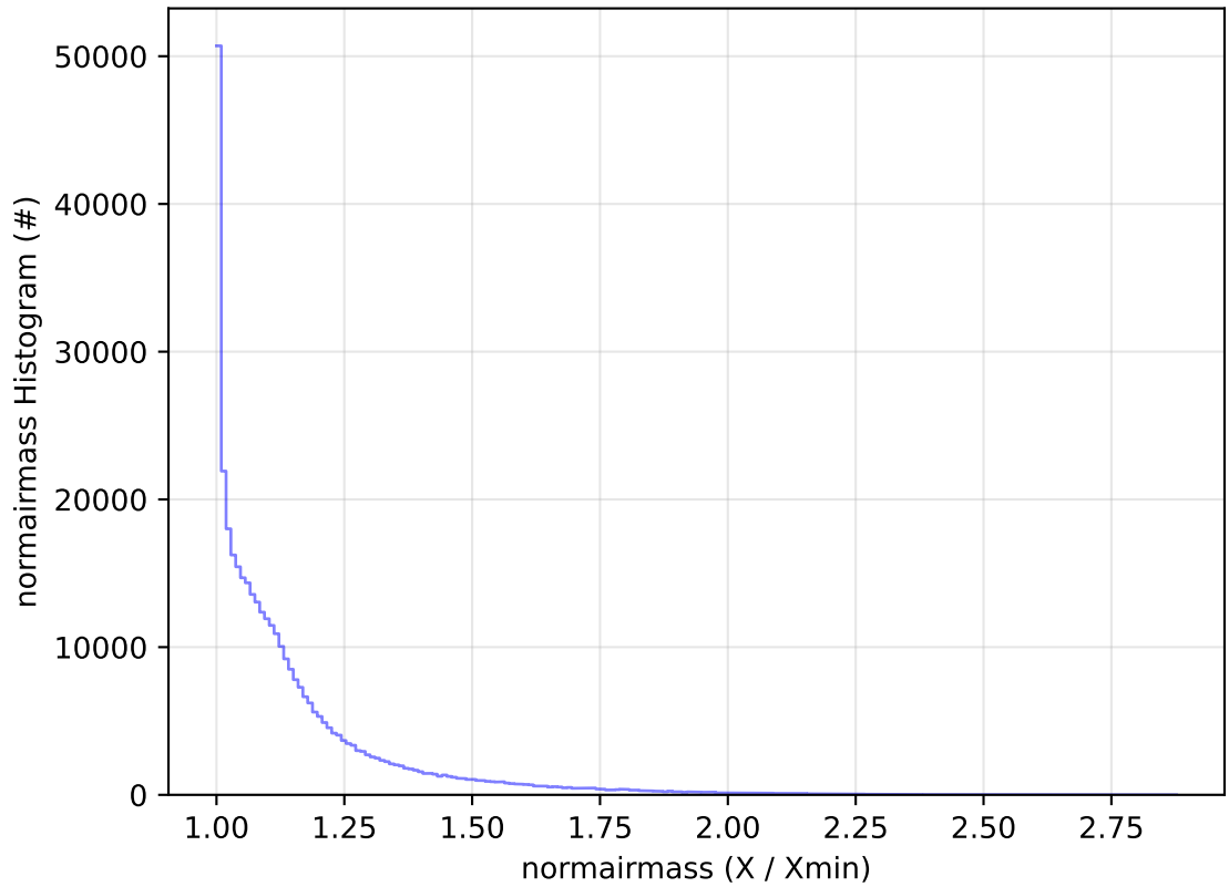
ddf_acor_sf10_lsf15_lsr10_v3.4_10yrs All sky y band: normairmass Histogram
