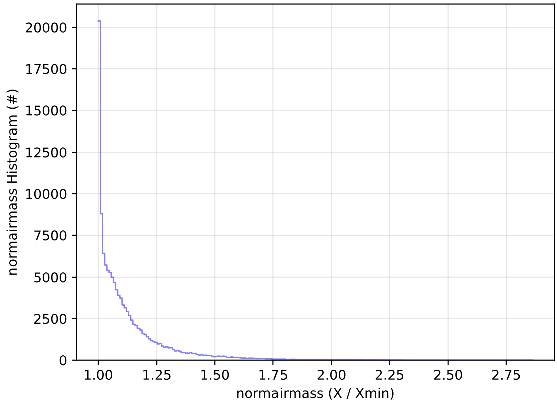
ddf_acor_sf10_lsf15_lsr10_v3.4_10yrs All sky u band: normairmass Histogram
