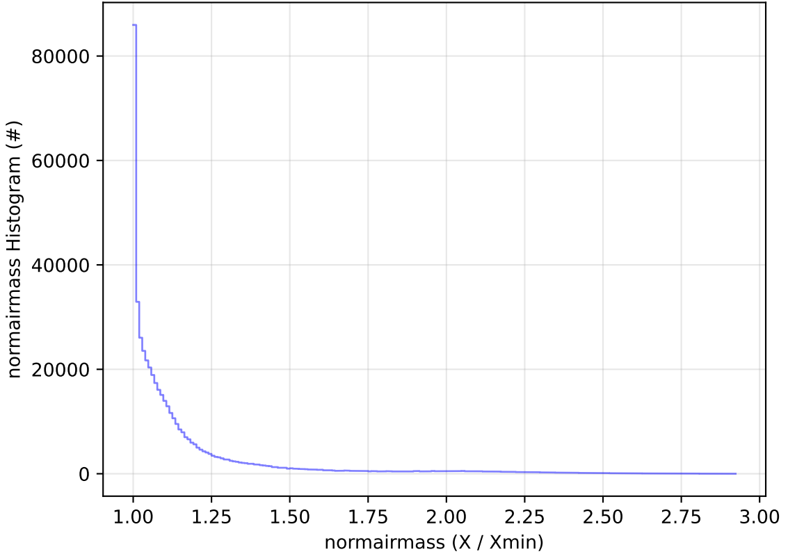
ddf_acor_sf10_lsf15_lsr10_v3.4_10yrs All sky i band: normairmass Histogram
