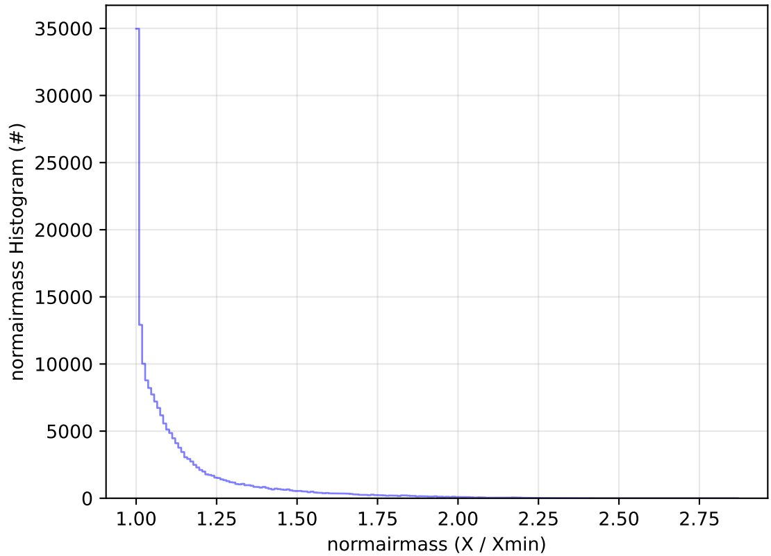
ddf_acor_sf10_lsf15_lsr10_v3.4_10yrs All sky g band: normairmass Histogram
