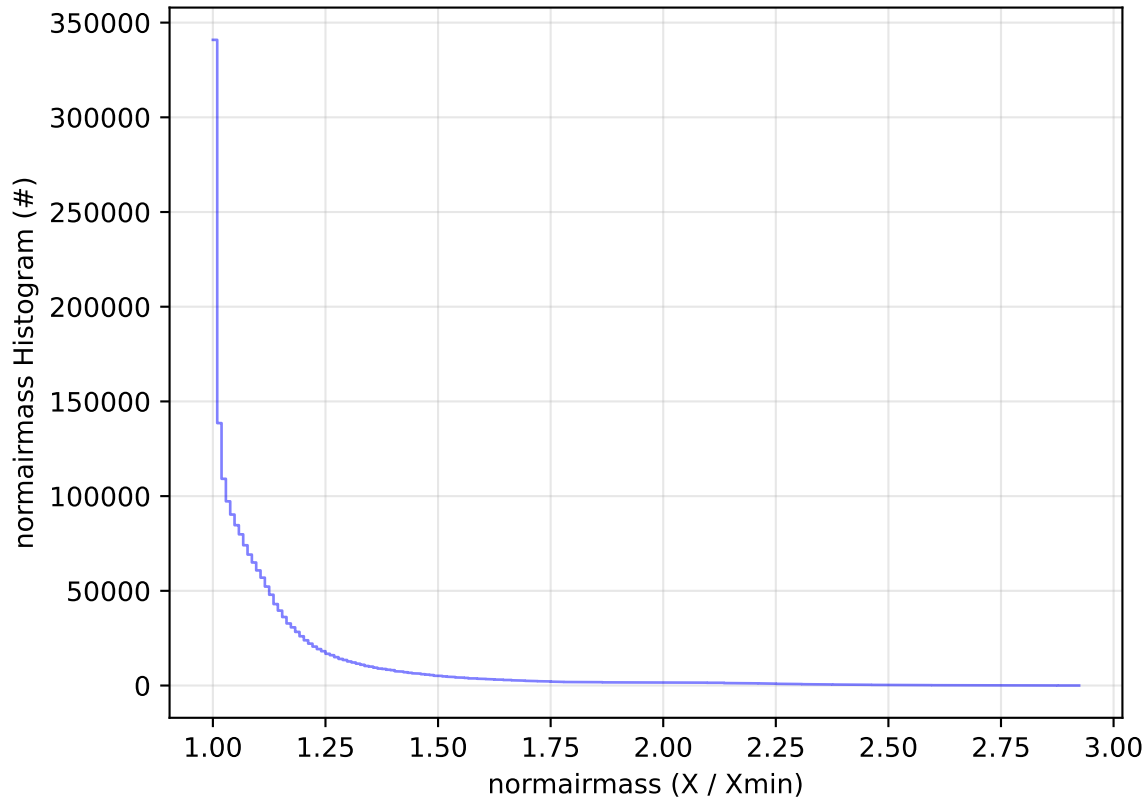
ddf_acor_sf10_lsf15_lsr10_v3.4_10yrs All sky all bands: normairmass Histogram
