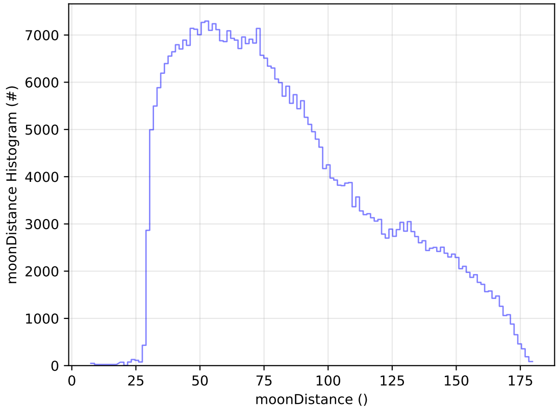
ddf_acor_sf10_lsf15_lsr10_v3.4_10yrs WFD z band: moonDistance Histogram
