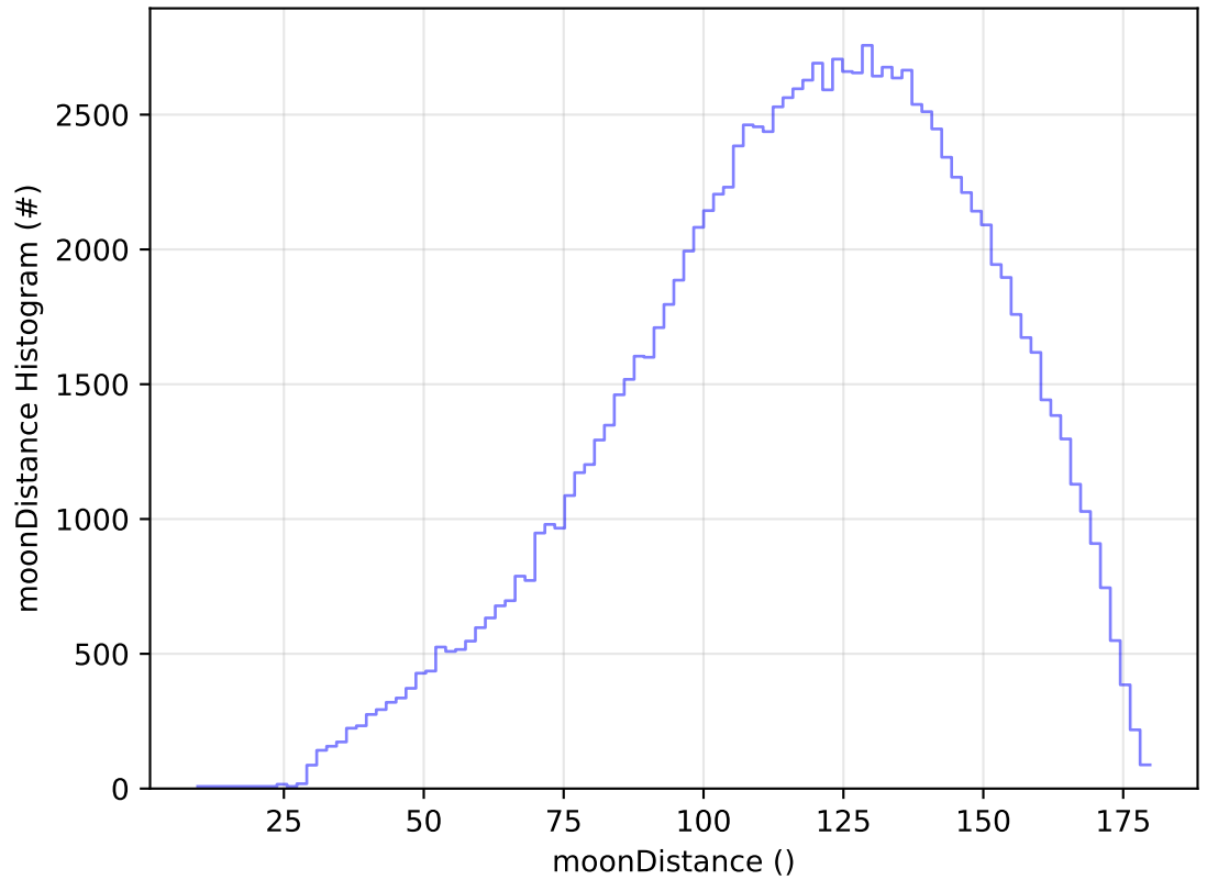
ddf_acor_sf10_lsf15_lsr10_v3.4_10yrs WFD u band: moonDistance Histogram
