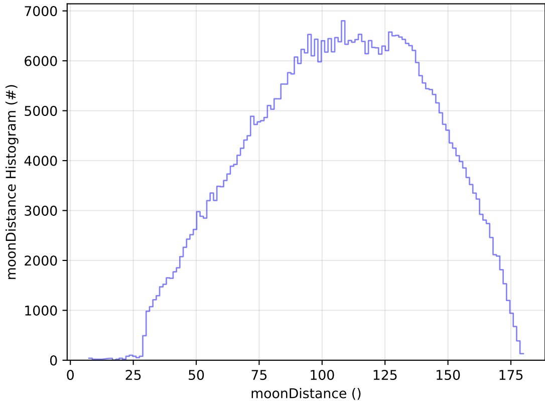
ddf_acor_sf10_lsf15_lsr10_v3.4_10yrs WFD r band: moonDistance Histogram
