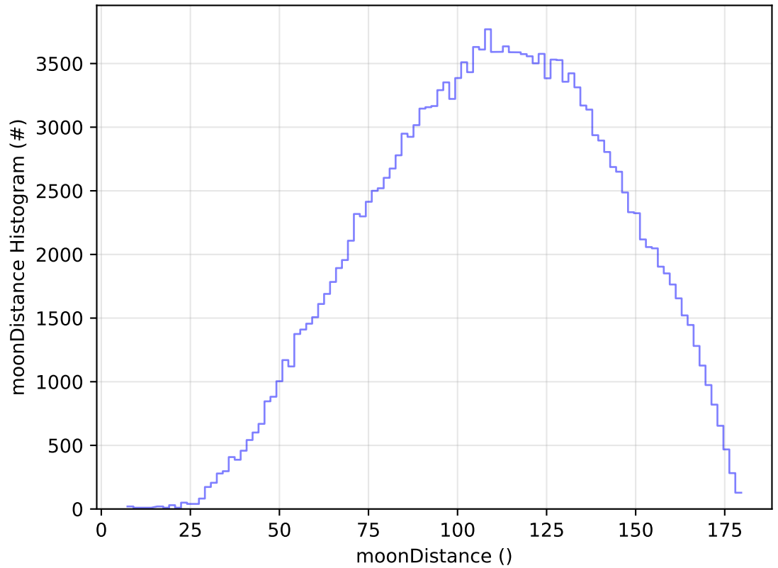
ddf_acor_sf10_lsf15_lsr10_v3.4_10yrs WFD g band: moonDistance Histogram
