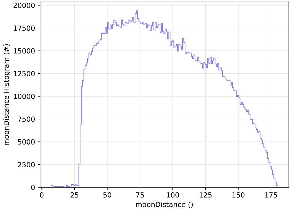
ddf_acor_sf10_lsf15_lsr10_v3.4_10yrs WFD all bands: moonDistance Histogram
