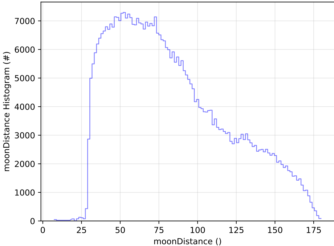
ddf_acor_sf10_lsf15_lsr10_v3.4_10yrs All sky z band: moonDistance Histogram
