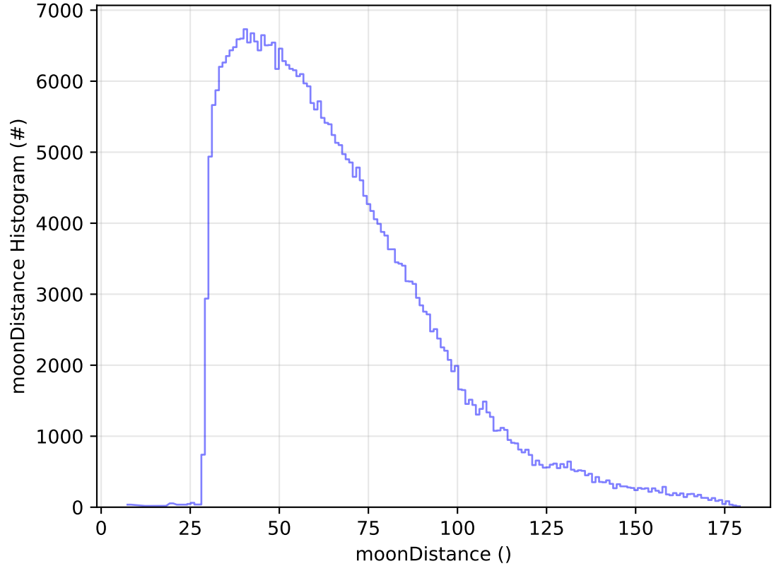
ddf_acor_sf10_lsf15_lsr10_v3.4_10yrs All sky y band: moonDistance Histogram
