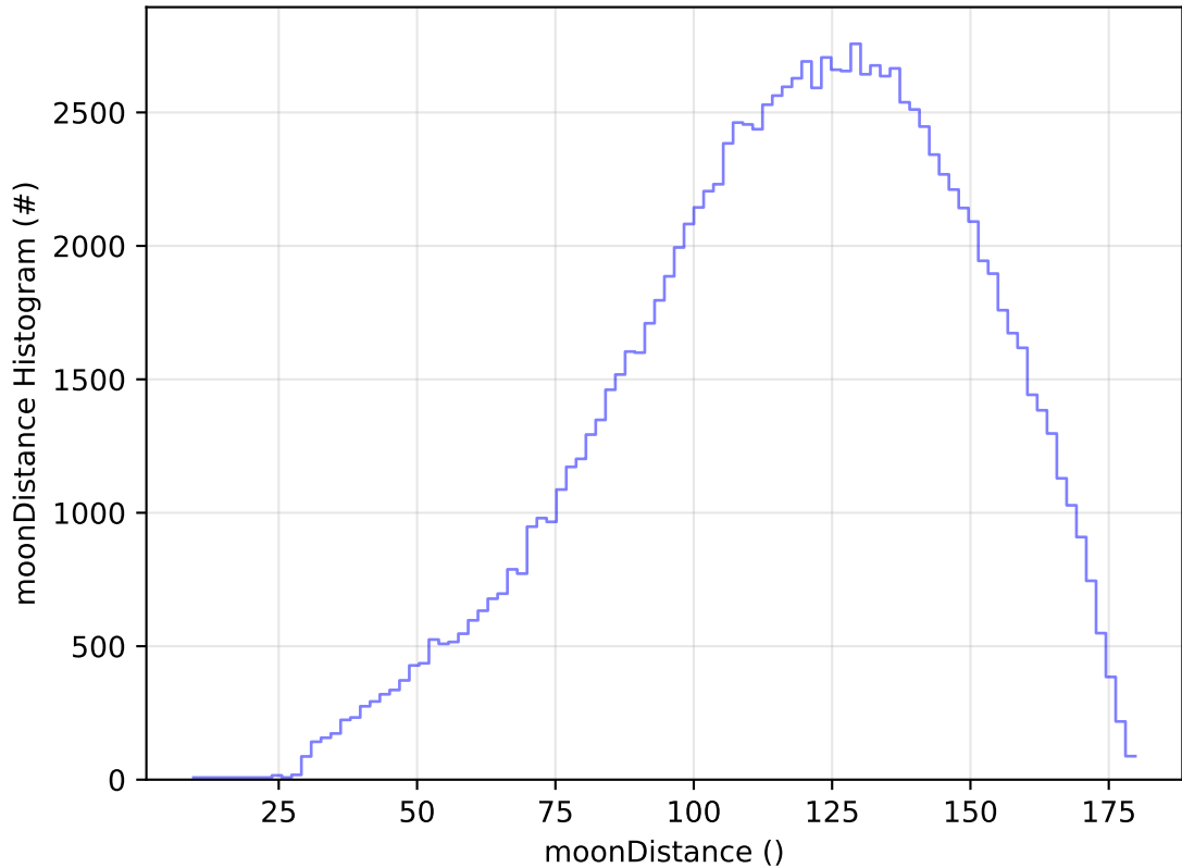
ddf_acor_sf10_lsf15_lsr10_v3.4_10yrs All sky u band: moonDistance Histogram
