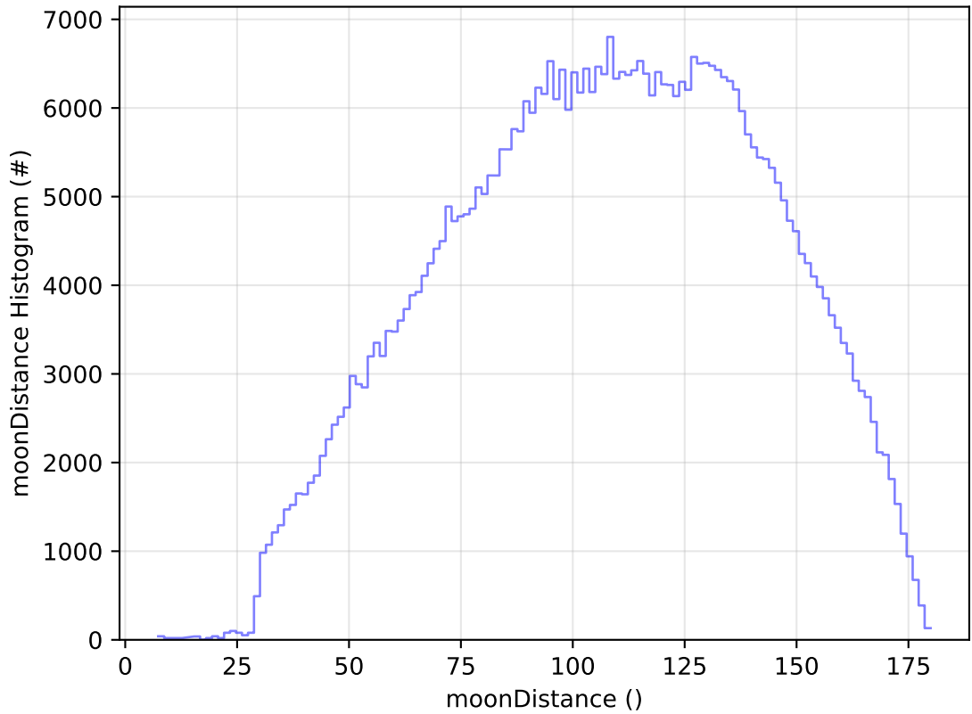
ddf_acor_sf10_lsf15_lsr10_v3.4_10yrs All sky r band: moonDistance Histogram
