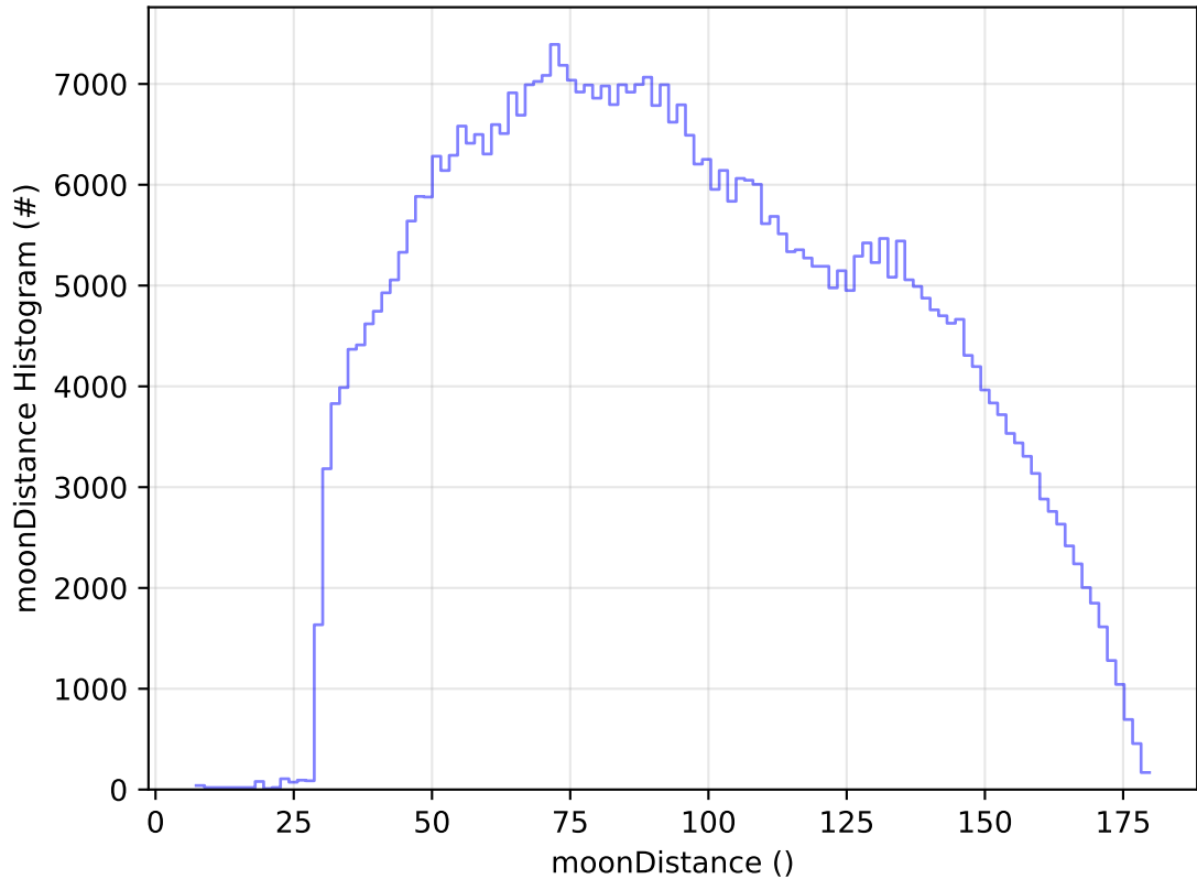
ddf_acor_sf10_lsf15_lsr10_v3.4_10yrs All sky i band: moonDistance Histogram
