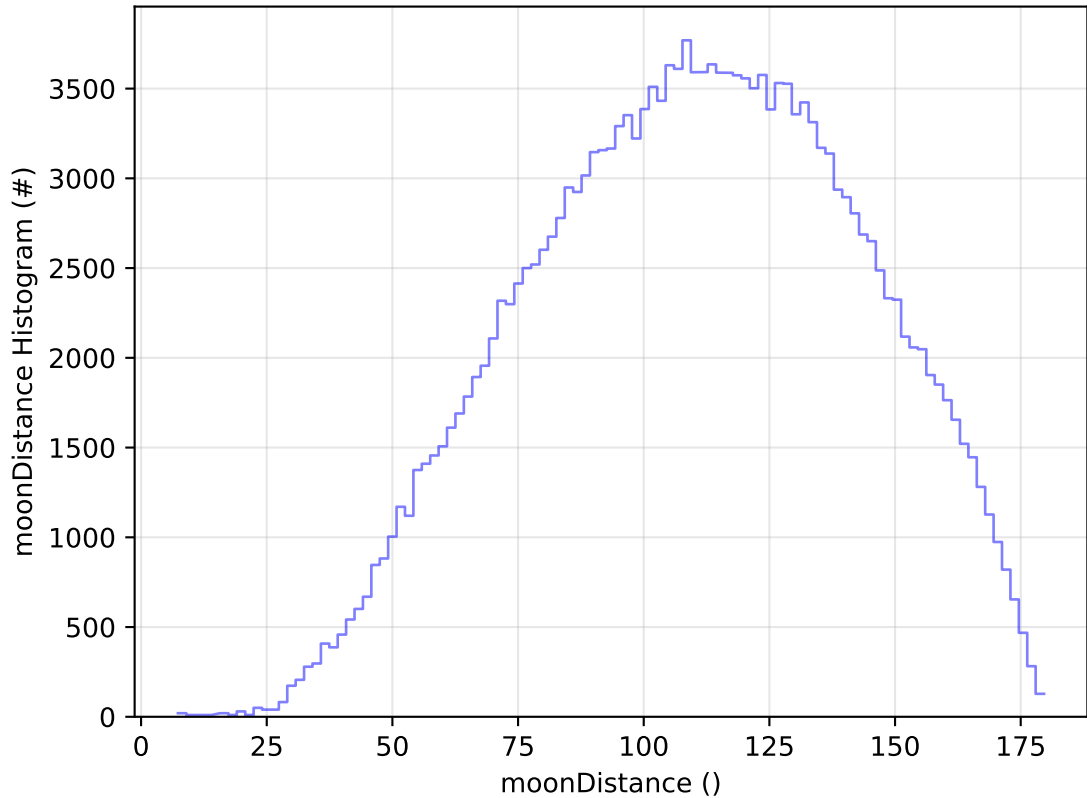
ddf_acor_sf10_lsf15_lsr10_v3.4_10yrs All sky g band: moonDistance Histogram
