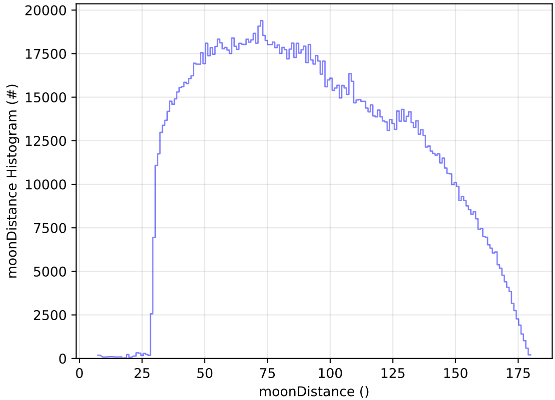
ddf_acor_sf10_lsf15_lsr10_v3.4_10yrs All sky all bands: moonDistance Histogram
