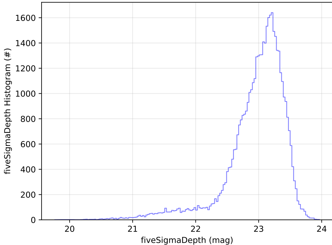
ddf_acor_sf10_lsf15_lsr10_v3.4_10yrs Yr 1 z band: fiveSigmaDepth Histogram
