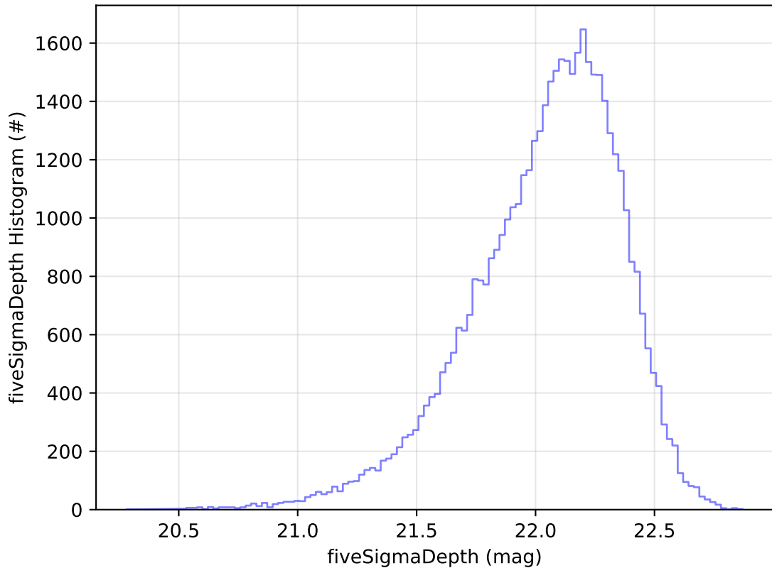
ddf_acor_sf10_lsf15_lsr10_v3.4_10yrs Yr 1 y band: fiveSigmaDepth Histogram
