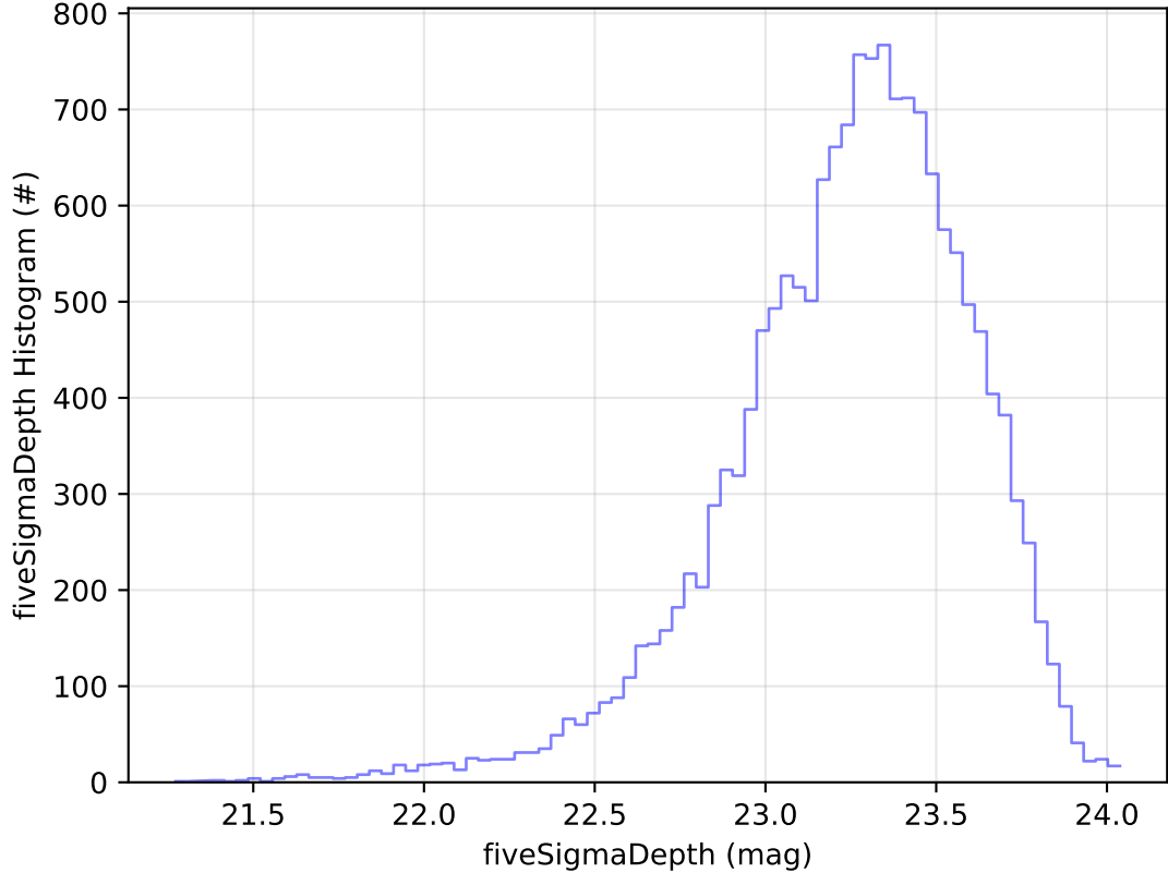
ddf_acor_sf10_lsf15_lsr10_v3.4_10yrs Yr 1 u band: fiveSigmaDepth Histogram
