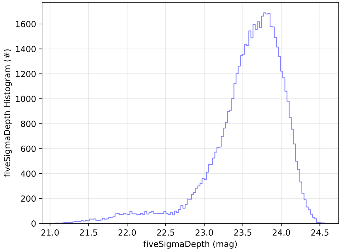
ddf_acor_sf10_lsf15_lsr10_v3.4_10yrs Yr 1 i band: fiveSigmaDepth Histogram
