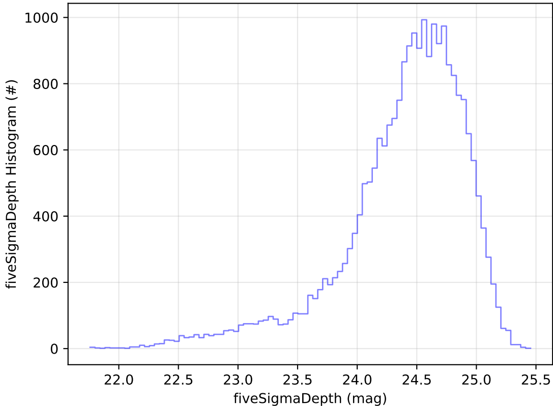
ddf_acor_sf10_lsf15_lsr10_v3.4_10yrs Yr 1 g band: fiveSigmaDepth Histogram
