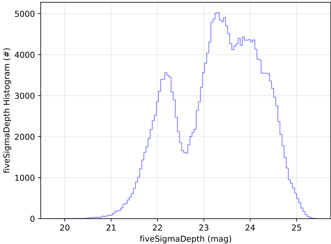
ddf_acor_sf10_lsf15_lsr10_v3.4_10yrs Yr 1 all bands: fiveSigmaDepth Histogram
