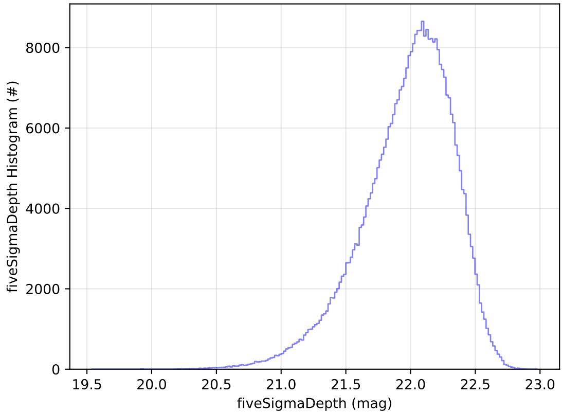
ddf_acor_sf10_lsf15_lsr10_v3.4_10yrs WFD y band: fiveSigmaDepth Histogram
