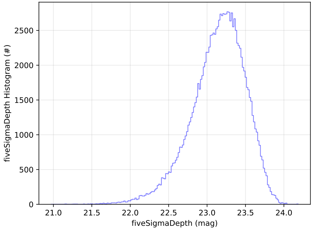
ddf_acor_sf10_lsf15_lsr10_v3.4_10yrs WFD u band: fiveSigmaDepth Histogram
