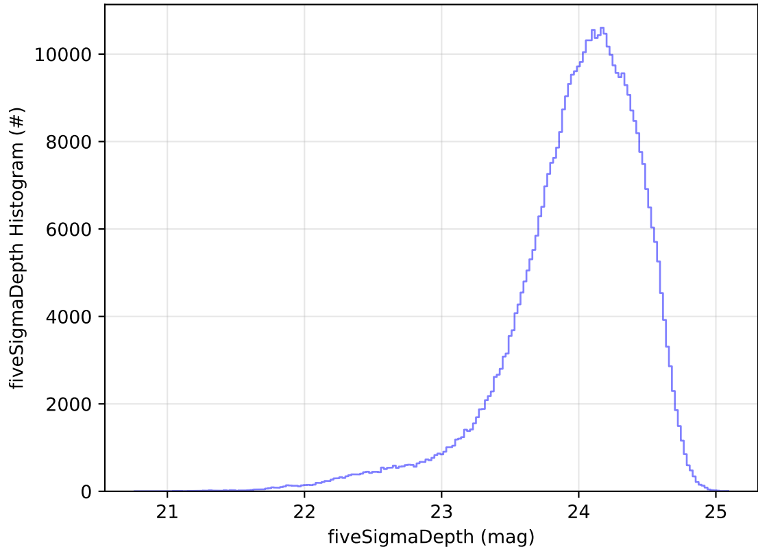
ddf_acor_sf10_lsf15_lsr10_v3.4_10yrs WFD r band: fiveSigmaDepth Histogram
