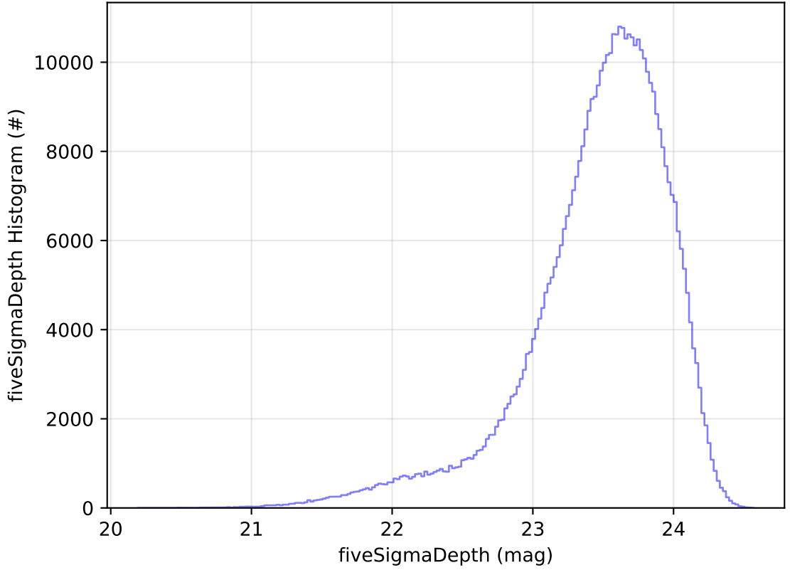
ddf_acor_sf10_lsf15_lsr10_v3.4_10yrs WFD i band: fiveSigmaDepth Histogram
