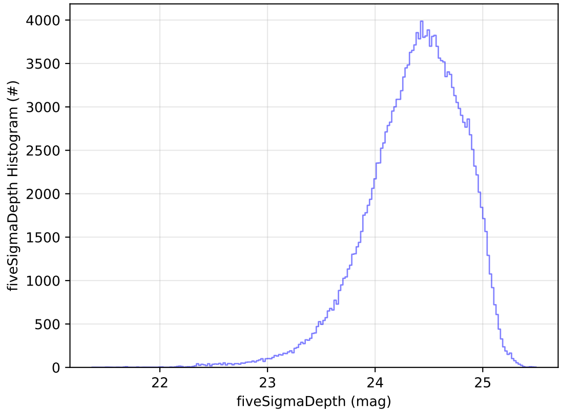
ddf_acor_sf10_lsf15_lsr10_v3.4_10yrs WFD g band: fiveSigmaDepth Histogram
