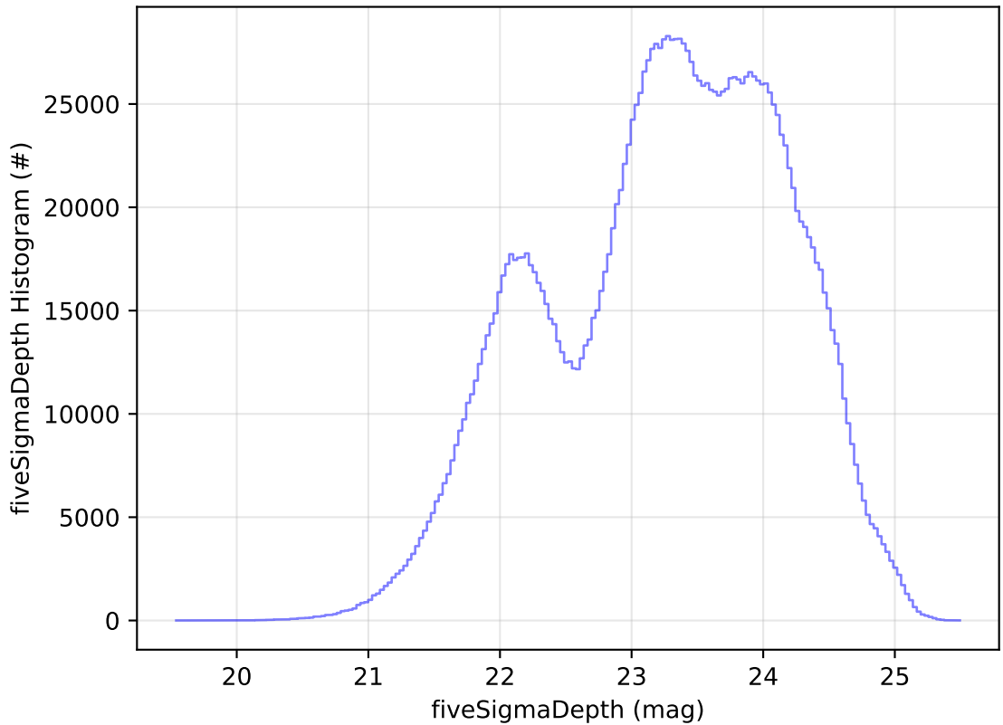
ddf_acor_sf10_lsf15_lsr10_v3.4_10yrs WFD all bands: fiveSigmaDepth Histogram
