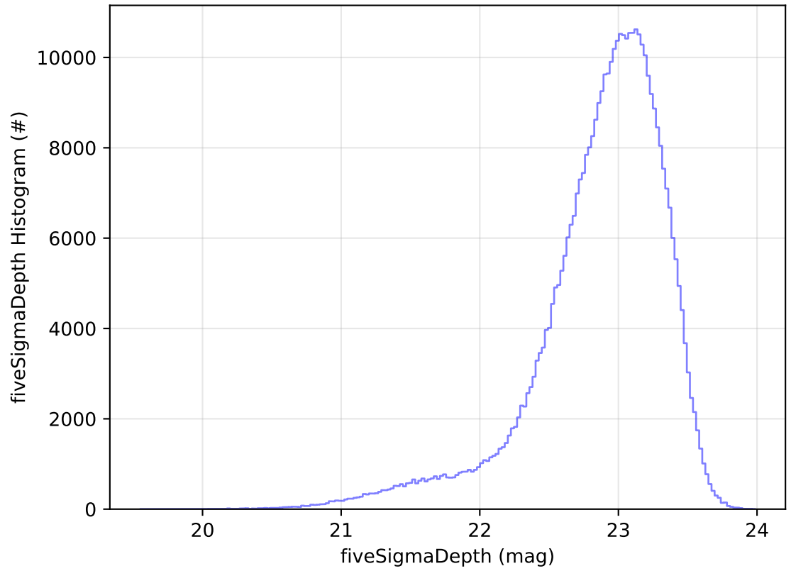
ddf_acor_sf10_lsf15_lsr10_v3.4_10yrs All sky z band: fiveSigmaDepth Histogram
