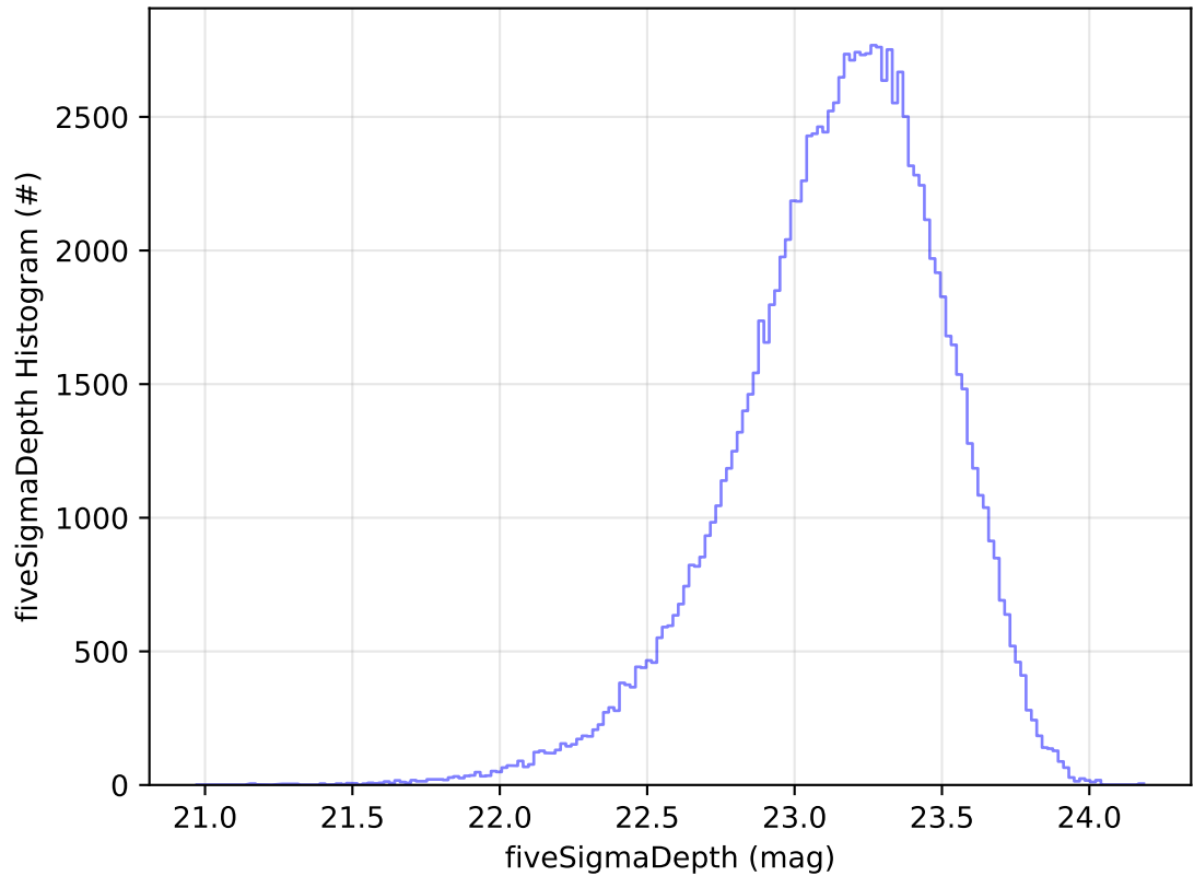
ddf_acor_sf10_lsf15_lsr10_v3.4_10yrs All sky u band: fiveSigmaDepth Histogram
