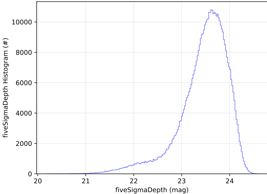
ddf_acor_sf10_lsf15_lsr10_v3.4_10yrs All sky i band: fiveSigmaDepth Histogram
