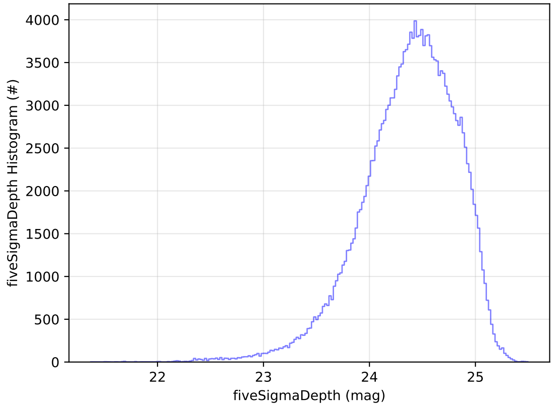
ddf_acor_sf10_lsf15_lsr10_v3.4_10yrs All sky g band: fiveSigmaDepth Histogram
