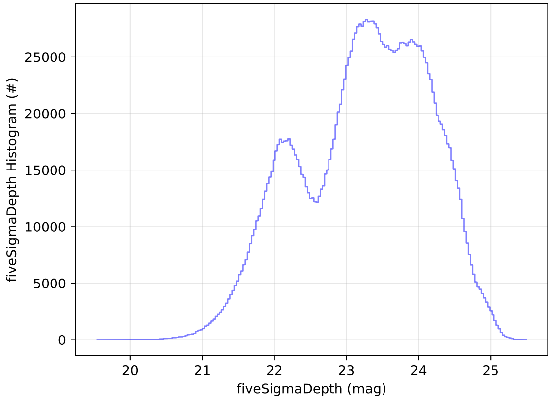
ddf_acor_sf10_lsf15_lsr10_v3.4_10yrs All sky all bands: fiveSigmaDepth Histogram
