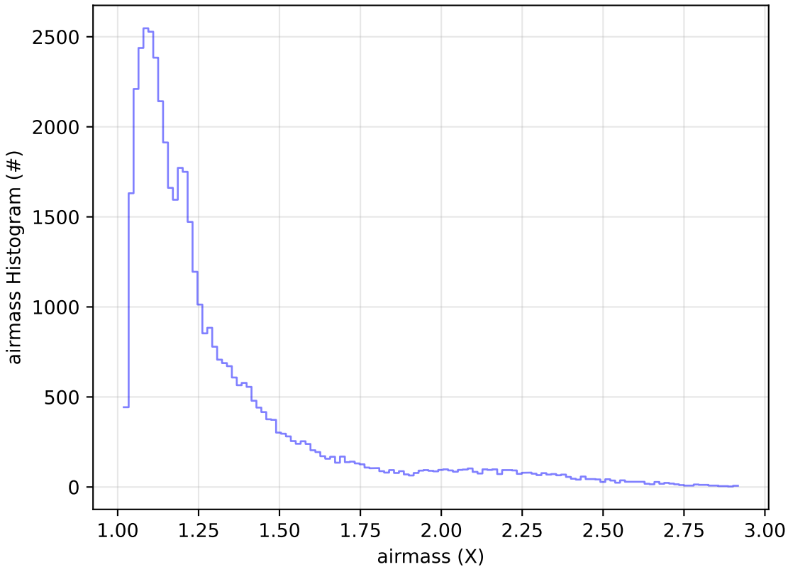
ddf_acor_sf10_lsf15_lsr10_v3.4_10yrs Yr 1 z band: airmass Histogram
