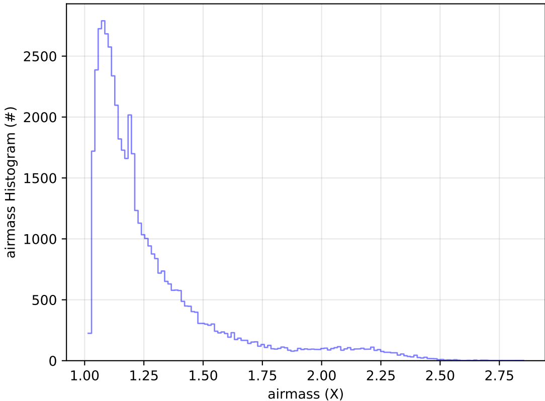
ddf_acor_sf10_lsf15_lsr10_v3.4_10yrs Yr 1 r band: airmass Histogram
