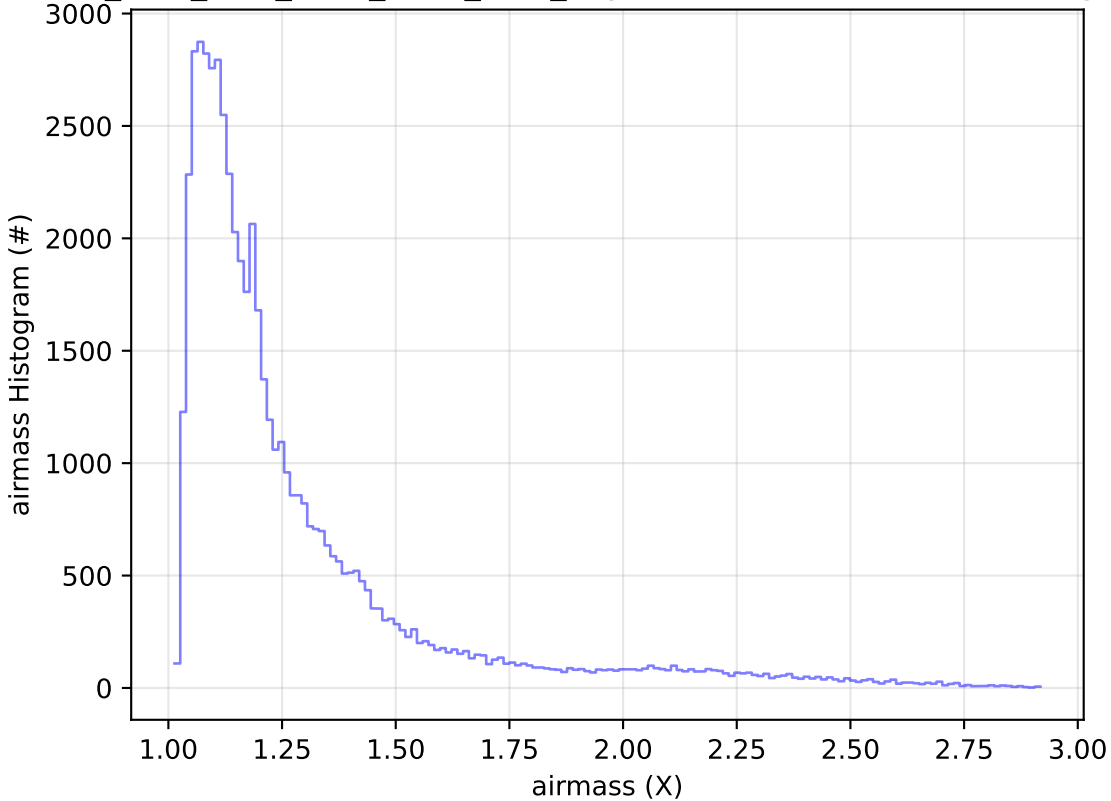
ddf_acor_sf10_lsf15_lsr10_v3.4_10yrs Yr 1 i band: airmass Histogram
