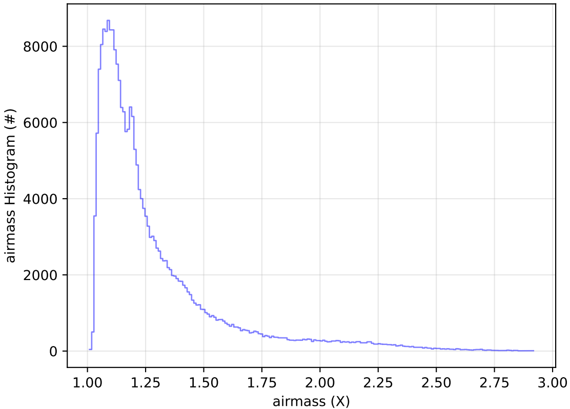
ddf_acor_sf10_lsf15_lsr10_v3.4_10yrs Yr 1 all bands: airmass Histogram
