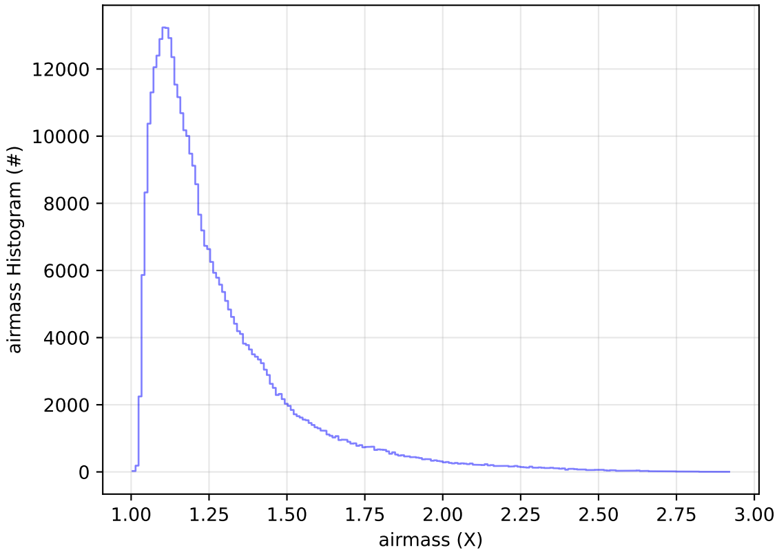
ddf_acor_sf10_lsf15_lsr10_v3.4_10yrs WFD y band: airmass Histogram
