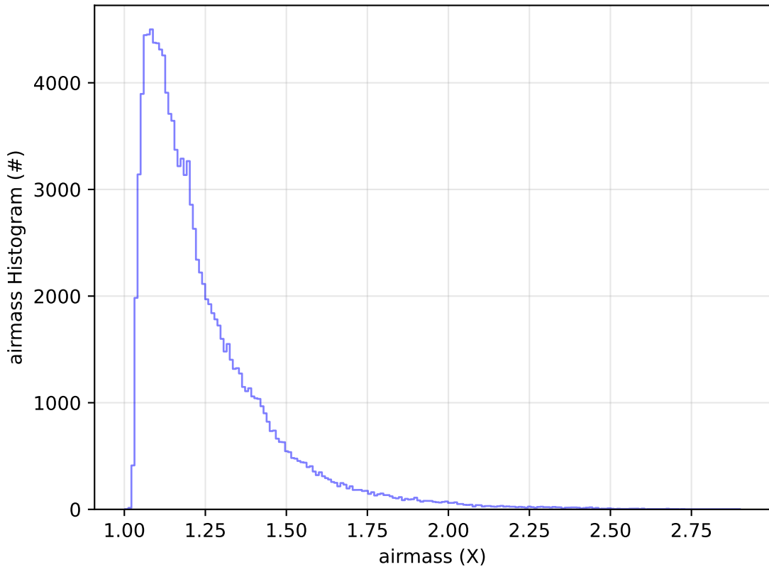
ddf_acor_sf10_lsf15_lsr10_v3.4_10yrs WFD u band: airmass Histogram
