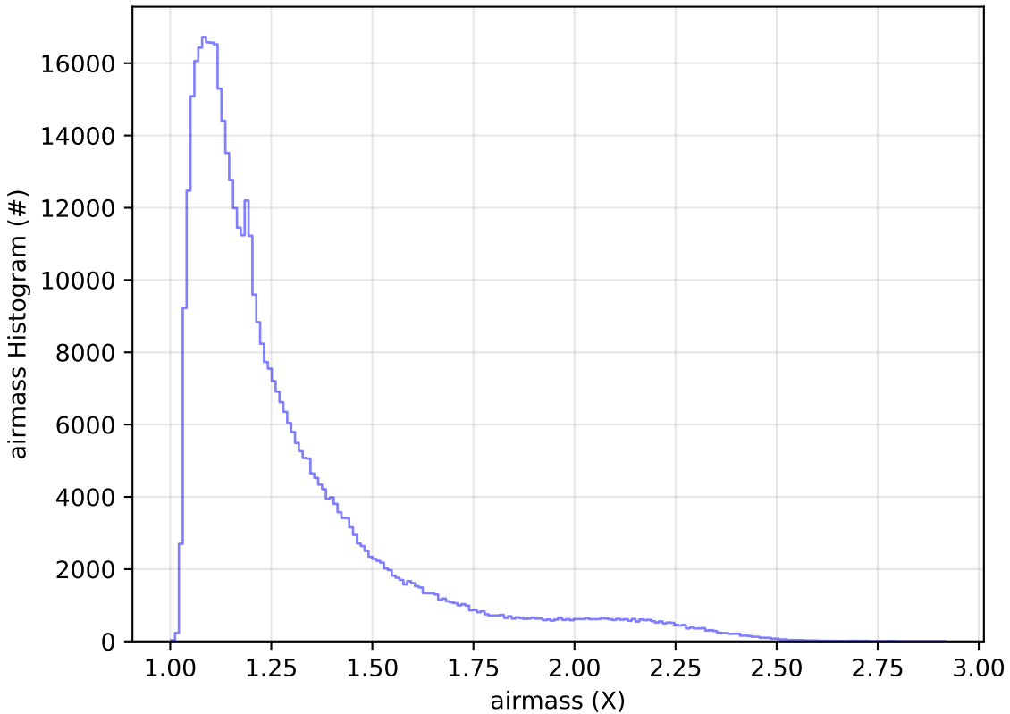
ddf_acor_sf10_lsf15_lsr10_v3.4_10yrs WFD r band: airmass Histogram
