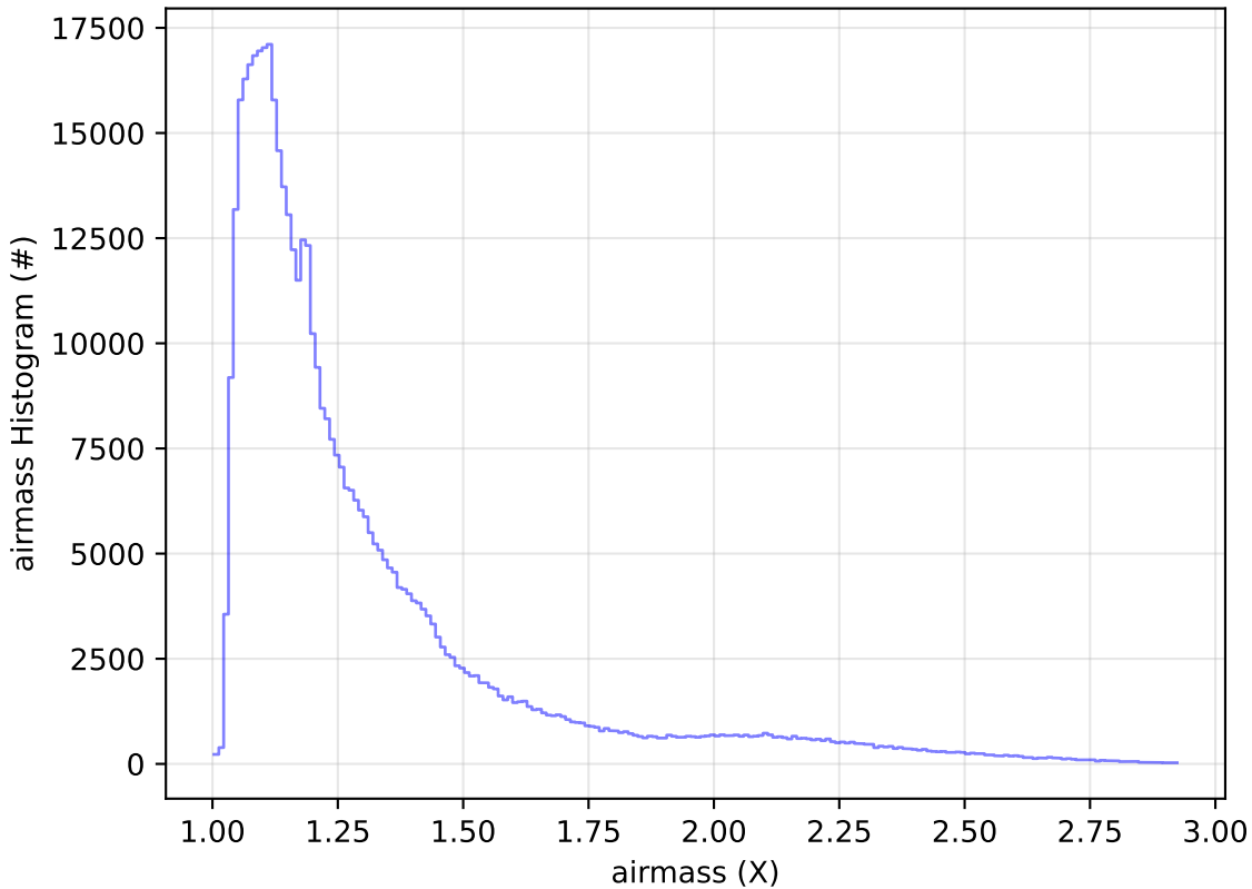
ddf_acor_sf10_lsf15_lsr10_v3.4_10yrs WFD i band: airmass Histogram
