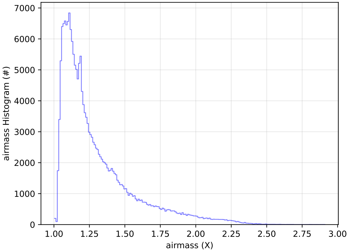
ddf_acor_sf10_lsf15_lsr10_v3.4_10yrs WFD g band: airmass Histogram
