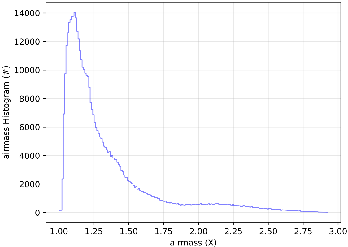
ddf_acor_sf10_lsf15_lsr10_v3.4_10yrs All sky z band: airmass Histogram
