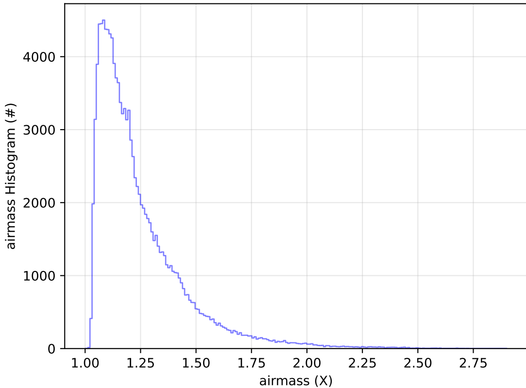
ddf_acor_sf10_lsf15_lsr10_v3.4_10yrs All sky u band: airmass Histogram
