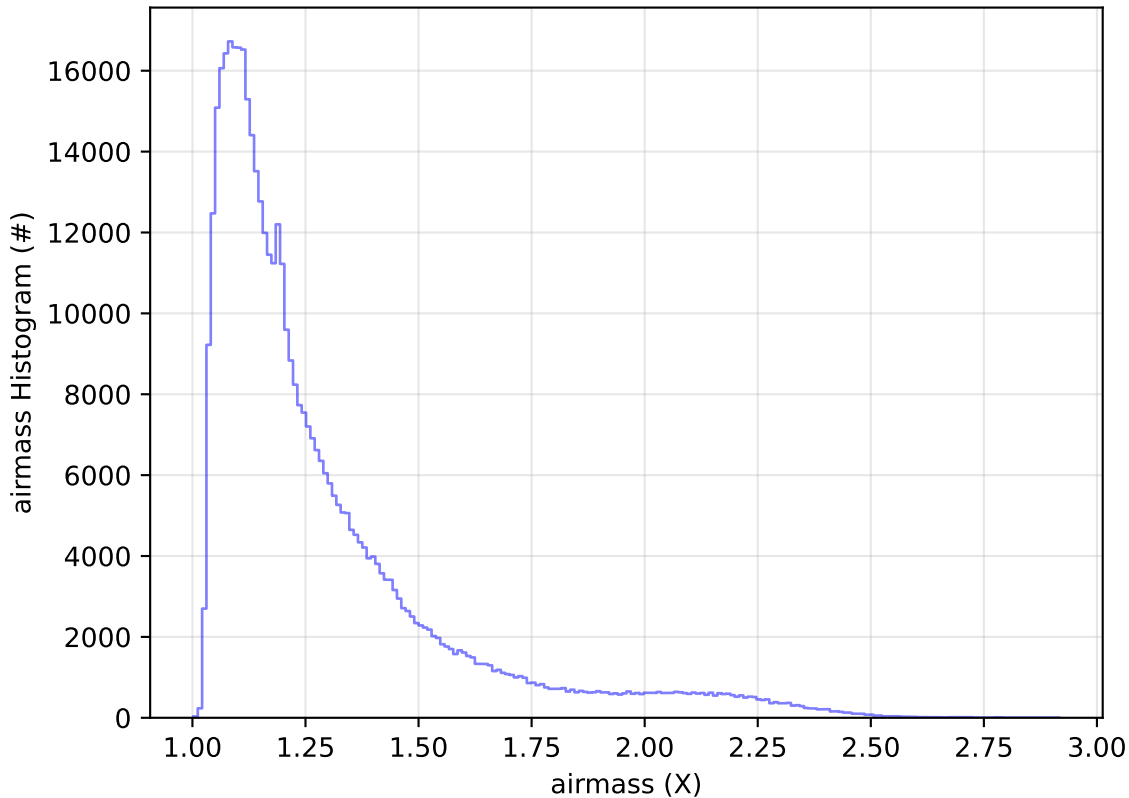
ddf_acor_sf10_lsf15_lsr10_v3.4_10yrs All sky r band: airmass Histogram
